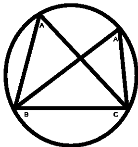
Fig. 3: Another maths sketch
