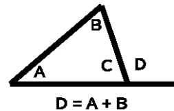
Fig. 2: A maths sketch
